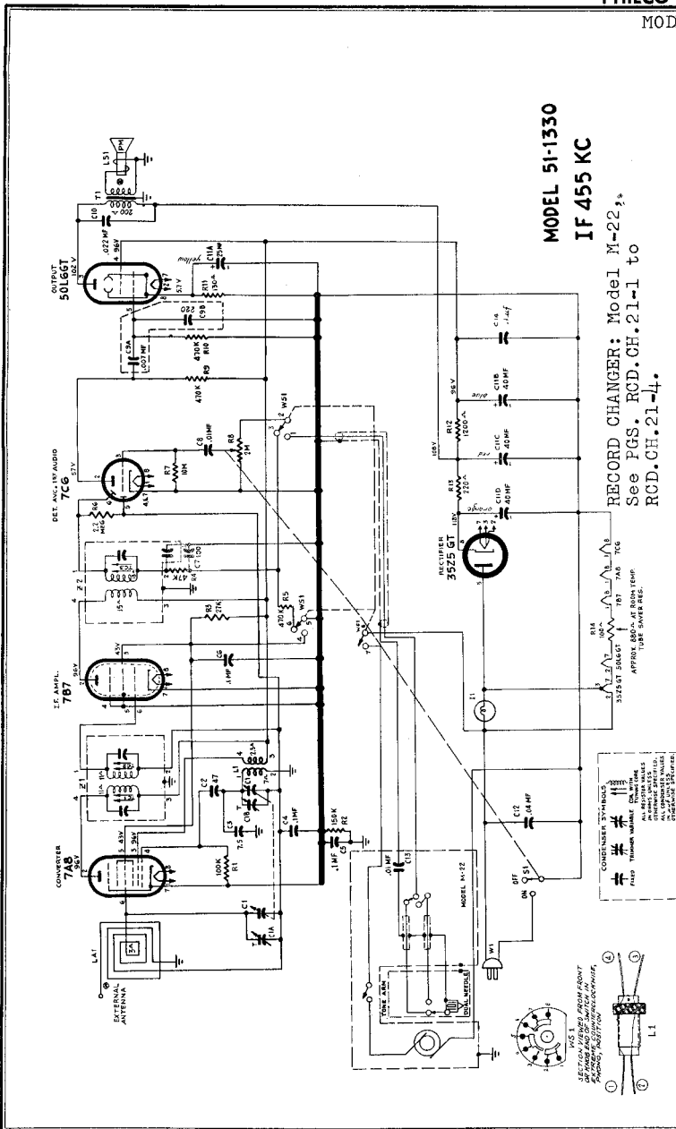
Figure 3. Philco Radio-Phonograph Model 51-1330, Schematic Diagram
