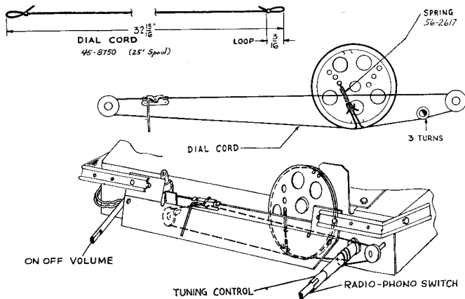
Figure 1. Drive-Cord Installation Details
