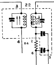
Figure 4. Run 2 I-F Transformer
