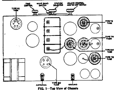
FIG. 1—Top View of Chassis
