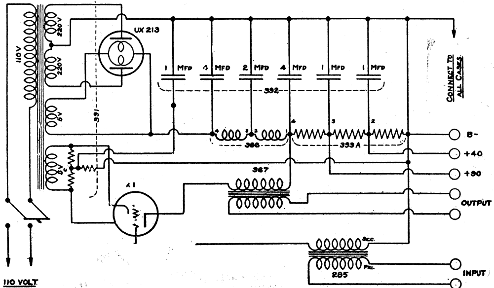
(Showing the schematic diagram of the Type 390 Rectron "B" Eliminator and Power Amplifier)
